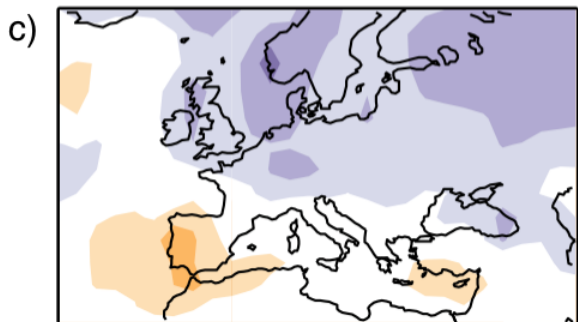
Low tropical amplification, weak vortex
