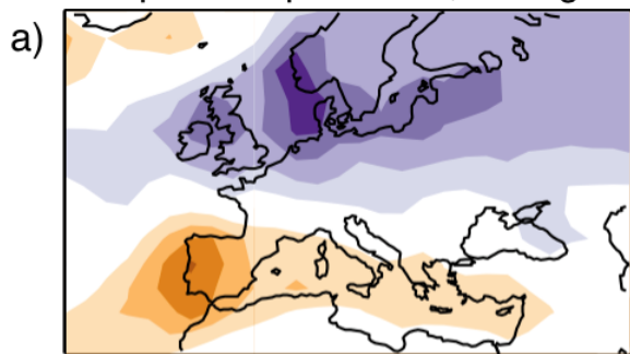
Low tropical amplification, weak vortex
